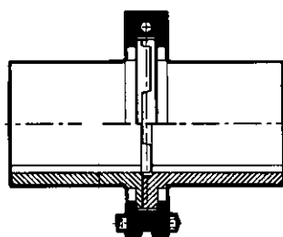
Quick Release Flanges
