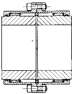
Gear Type Couplings
